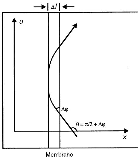
Fig. 3. Trajectory with greatest \theta that is still fully deflected back into right hand side of vessel.
