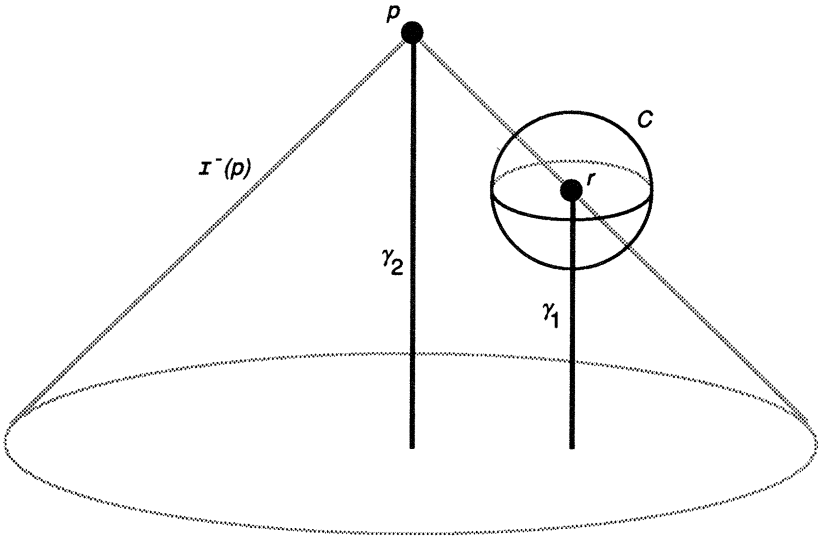
Figure 1. A Toy Malament-Hogarth Spacetime.
