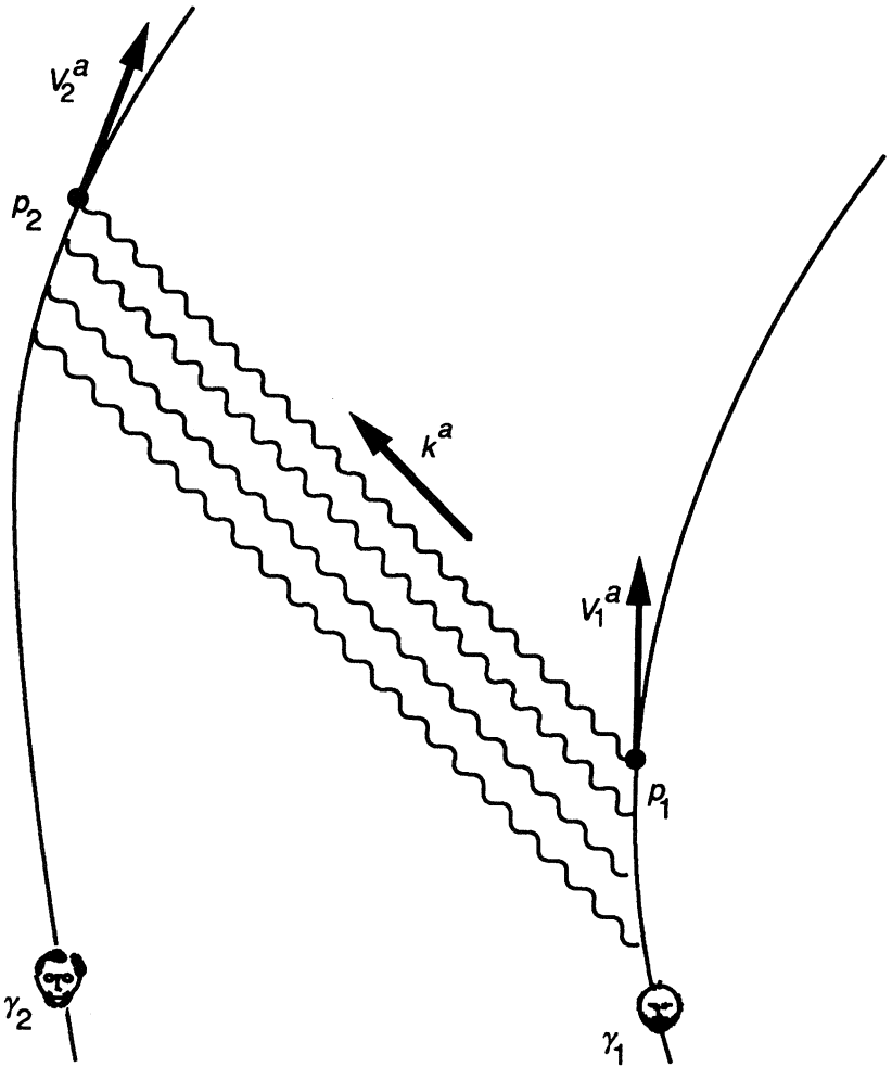
Figure 2. The Redshift/Blueshift Effect.
